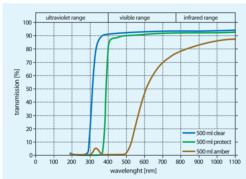
Light transmission curves for DURAN® glass (500 ml bottle)
