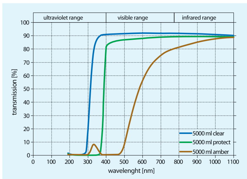
Light transmission curves for DURAN® glass (5 000 ml bottle)
